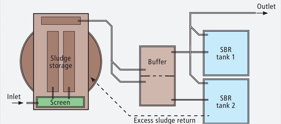
Plant layout:
