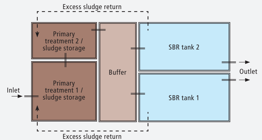
Plant layout:
